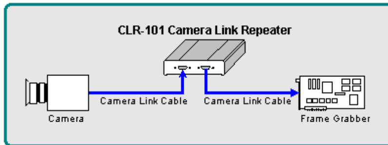
CLR-101 Connections
